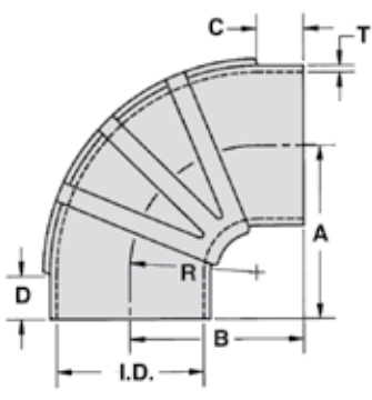
90° Elbow
