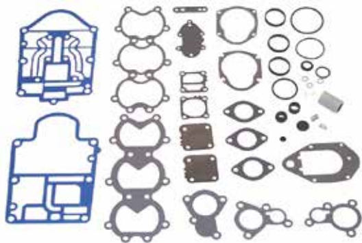
18-4337 POWERHEAD GASKET SET Replaces: 27-812867A97 For: 45 Jet, 50HP, 55HP, 60HP, 3 cyl outboards
