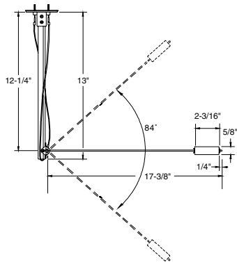
56948P Sender, Fuel, Kit, w/Gauge, 4-24" Tank
