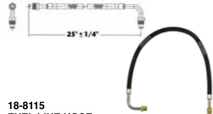
18-8115 FUEL LINE HOSE For fuel pump to carburetor connection. Replaces copper or steel tubing 3/8" X 25" PTFE composite hose with 5/8"-18 male inverted flare straight one end, 5/8"-18 90° one end. SAE J1527 type A1
