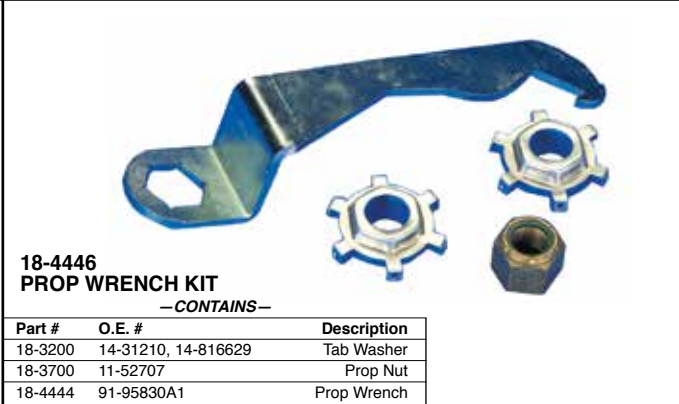
18-4444 PROP WRENCH Replaces: 91-95830A1
