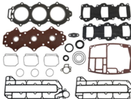
18-99176 POWERHEAD GASKET SET Replaces: 6H3-W0001-02 Fits: 60(2001-05), 70(1994-09), C70(2000-01), P60(1994-99)
