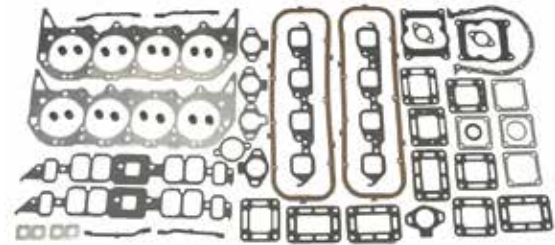
18-4365 EXHAUST MANIFOLD GASKET SET Replaces: 27-801855 For: GM 454 (7.4L) CID Eng; Production Models Rectangular Port Includes 18-3877 Head Gasket
