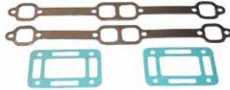
18-0604 EXHAUST MANIFOLD GASKET SET For: GM 305/350 CID Engines For use with 18-1997-1
