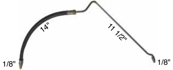
POWER TRIM HOSE Starboard Connector to bottom of trim cylinder MCM 120-260 & BRAVO
