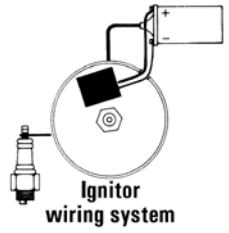
18-5289 HI-PERFORMANCE ELECTRONIC CONVERSION KIT Fits: Most Prestolite V-8 Distributors with screw down cap
