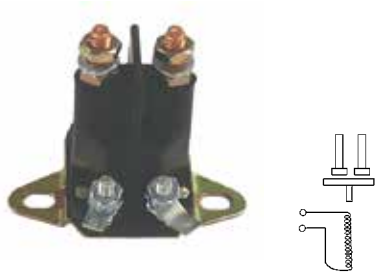
18-5810 SOLENOID
