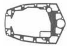
18-99025 UPPER CASING GASKET Replaces: 688-45114-A1 Fits: 90(1984-09), B90(1997-99), C75(1994-99), C80(1997), C85(1991-96), C90(1997-01), CV85(1989-90), E75(1995-00), P75(1996-99)
