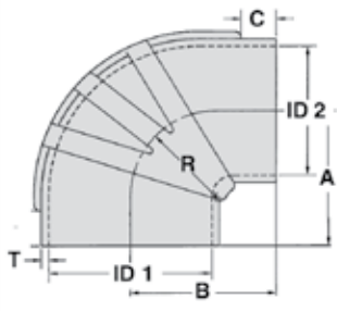
90° Reducing Elbow
