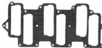
18-0807-1 REED PLATE GASKET Replaces: 6K7-13645-A1-00
