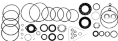
18-2625 STERNDRIVE GASKET KIT Replaces: 875192 AQ200, 250, 270, 275, 280, 290
