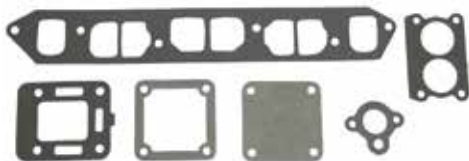
18-4367 EXHAUST MANIFOLD GASKET SET Replaces: 27-99777A1 For: GM 153 & 181 (2.5 & 3.0L) CID Eng's; 120 & 140 HP S/N 6229718 & UP (With Siamese Port Cylinder Heads)
