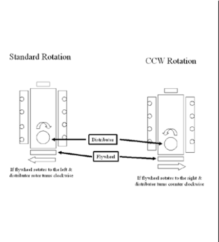
18-5480 COMPLETE IGNITION CONVERSION KIT Fits: GM SB & BB with Standard Deck Height
