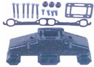
18-1986-1 MANIFOLD Port & Starboard Replaces: 3852374-2, 3857723, 3847501 For: 5.0L & 5.7L GM (New Style) Use with: Exhaust Manifold Gasket: 18-2949 Mounting Kit: 18-8502
