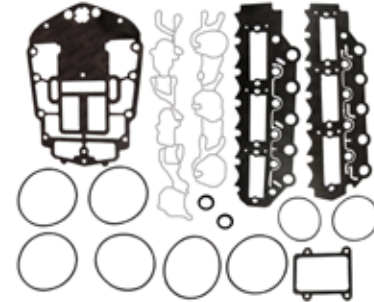
18-4406 POWERHEAD GASKET SET Replaces: 437155 Fits: 150 60 degree (1991-00), 175 60 degree (1991-00)
