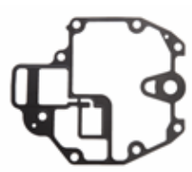
18-99027 OIL PAN GASKET Replaces: 68T-13475-00 Fits: F6(2001-08), F8(2001-10), F9.9(2007, 2010), T8(2001-10), T9.9(2007-10)
