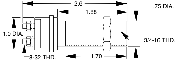
1507678P Mag. Prox. Sender
