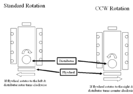
18-5299 ELECTRONIC CONVERSION KIT (with screw down cap) For: Most Prestolite V-8 Distributors Use with 18-5403 style rotor
