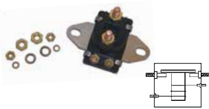
18-5816 SOLENOID Replaces: 89-96054, T, 89-91975 (Flat Bracket)
