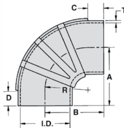
90° Elbow
