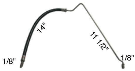
POWER TRIM HOSE Starboard Connector to bottom of trim cylinder MCM 120-260 & BRAVO
