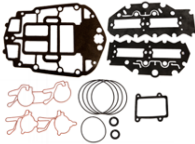
18-4402 POWERHEAD GASKET SET Replaces: 437779 Fits: 90 V4 60 degree (1995-00), 115 V4 60 degree (1995-00)
