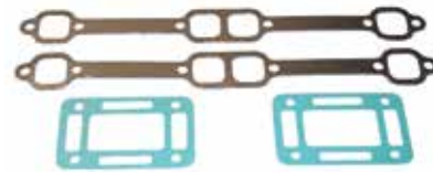
18-0604 EXHAUST MANIFOLD GASKET SET Use with: Manifold: 18-1997-1 For: GM 305/350 CID Engines
