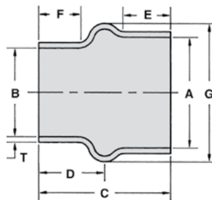
Hump Hose
