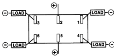
MOM ON-OFF-MOM ON DPDT
