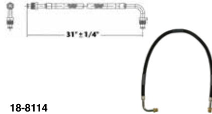
18-8114 FUEL LINE HOSE For fuel pump to carburetor connection. Replaces copper or steel tubing 3/8" X 31" PTFE composite hose with 5/8"-18 male inverted flare straight one end, 5/8"-18 90° one end. SAE J1527 type A1
