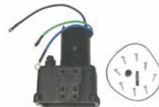
18-6763 TILT/TRIM MOTOR Replaces: 92975A6, 79271A4, 67914A2, 92975A32, 93247A7 To 1984. Fits most Mercruiser Sterndrives (Motor and Reservoir Only) For Repair Kit use: 18-6253
