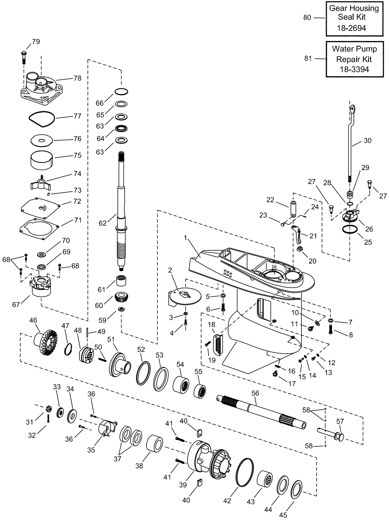
Complete Gear Housings Listed on Page 276
