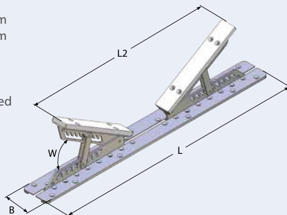
Tender- und Jetskihalter, variabel / Alu Tender and Jetski holder, variable
